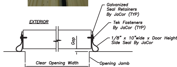
Detail B – TearDropSeal Bifold/Hydraulic Door Side Seal Detail
