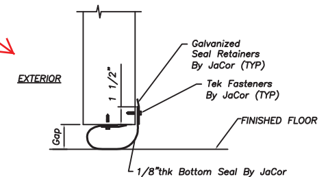
Detail A – BulbSeal Bifold/Hydraulic Door Bottom Seal Detail
