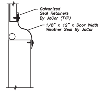
Detail C – CloseOffSeal Bifold/Hydraulic Door Top Seal Detail
